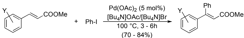
Scheme 5. Heck arylation of methyl 3-arylacrylates with iodobenzene.
