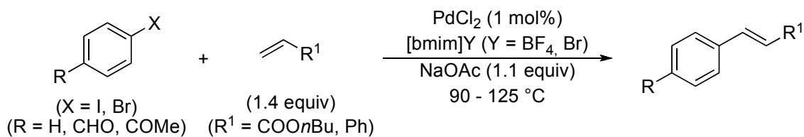
Scheme 19. Heck reaction in imidazolium based ILs.
