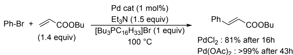
Scheme 1. Heck reaction without additive ligands in [C 16 PBu 3 ]Br.
