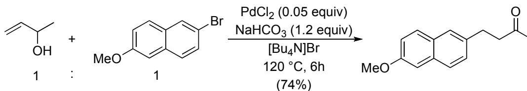
Scheme 7. Synthesis of nabumethone.
